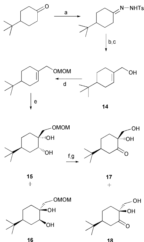
Scheme 4 Synthetic route for carba-analogues 17 and 18 . Reagents and yields : a, TsNHNH 2 , MeOH, H + , 99%; b, n -BuLi, THF, -78 °C; c, CH 2 O, 26% overall; d, CH 2 (OMe) 2 , LiBr-TsOH, 81%; e, K 2 OsO 4 -K 3 Fe(CN) 6 , MeSO 2 NH 2 , t -BuOH-H 2 O, 97%; f, Dess-Martin ox.; g, HCl-MeOH, 74–79% overall.
