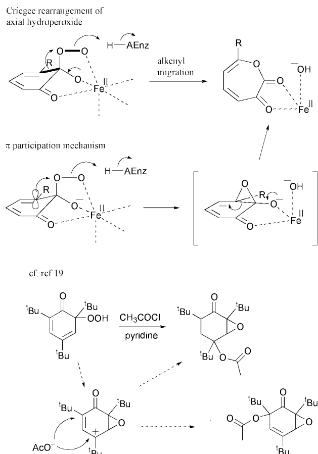
Fig. 5 Mechanisms for alkenyl migration of an axial proximal hydroperoxide intermediate, either via Criegee rearrangement ( \sigma bond migration) or participation of diene \pi system. Literature precedent for the latter mechanism (see ref. 19) is illustrated.
