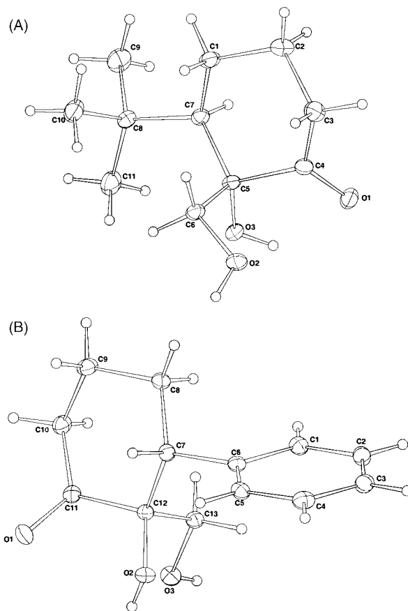
Fig. 2 X-Ray crystal structures of carba-analogues 10b (A) and 10c (B).
