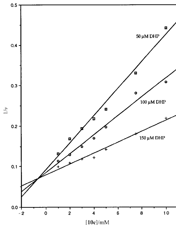
Fig. 3 Dixon plot 16 showing inhibition of E. coli 2,3-dihydroxyphenylpropionate 1,2-dioxygenase (MhpB) by carba-analogue 10c . Assays were carried out at 50, 100, and 150 \mu M concentrations of 2,3-dihydroxyphenylpropionic acid (DHP), as indicated. The point of intersection of the lines gives a K_i value of 0.7 mM.
