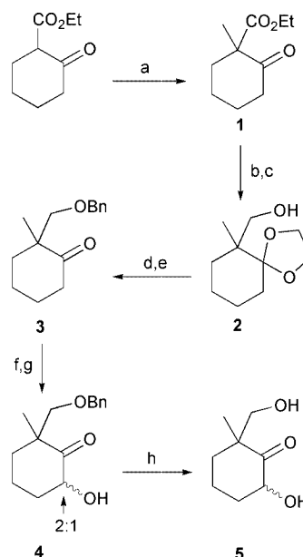
Scheme 1 Synthetic route for distal carba-analogue ( 5 ). Reagents and yields: a, t -BuOK–MeI, Aliquat 336, 97%; b, HO(CH 2 ) 2 OH, H + , 63%; c, LiAlH 4 , THF, 90%; d, NaH, BnBr, THF, 61%; e, H + –acetone–H 2 O, 87%; f, KHMDS, THF, –78 °C; g, PhCH(O)NTs, 62% overall; h, H 2 –Pd–C, 85%.
