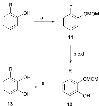
Scheme 3 Synthetic route of 3-substituted catechols 13a (R = Ph) and 13b (R = t -Bu). Reagents and yields (for 13b ): a, CH 3 OCH 2 Cl, NaH, THF, 89%; b, n -BuLi, THF, -78 °C; c, B(OMe) 3 ; d, Oxone, 65% overall; e, H + -H 2 O, 82%.
