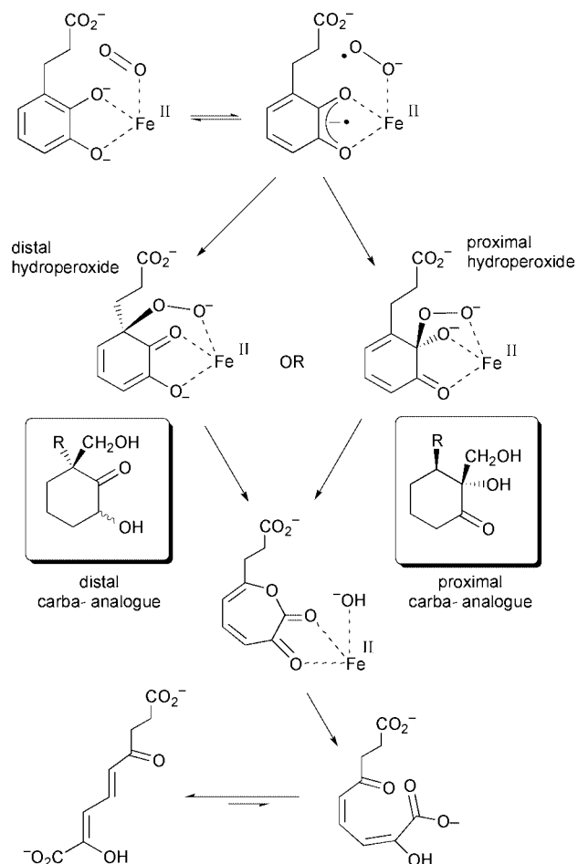
Fig. 1 Proposed catalytic mechanisms for 2,3-dihydroxyphenylpropionate 1,2-dioxygenase (MhpB), illustrating the proximal and distal hydroperoxide intermediates and their respective carba-analogues.
