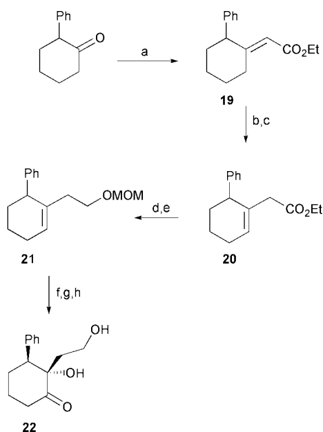
Scheme 5 Synthetic route for extended carba-analogue 22 . Reagents and yields : a, (EtO) 2 POCH 2 CO 2 Et, NaH, THF, 75%; b, LDA, THF, -78 °C; c, NH 4 Cl-H 2 O, 85% overall; d, LiAlH 4 , 96%; e, MOMCl, i -Pr 2 NEt, CH 2 Cl 2 , 94%; f, K 2 OsO 4 -K 3 Fe(CN) 6 , MeSO 2 NH 2 , t -BuOH-H 2 O, 98%; g, Dess-Martin ox.; h, HCl-MeOH, 42% overall.
