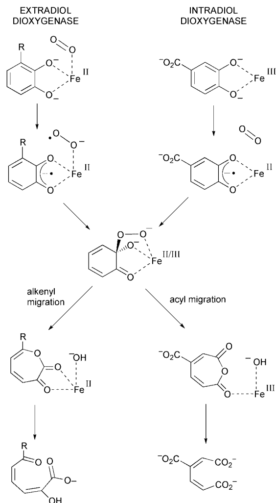
Fig. 4 Illustration of the convergence of the reaction mechanisms of the extradiol and intradiol catechol dioxygenases onto a similar proximal hydroperoxide intermediate, followed by divergence via alkenyl vs. acyl migration.
