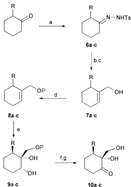
Scheme 2 Synthetic route for proximal carba-analogues 10a (R = CH 3 ), 10b (R = t -Bu), and 10c (R = Ph). P = protecting group: either TBDMS or MOM. Reagents and yields shown below:
